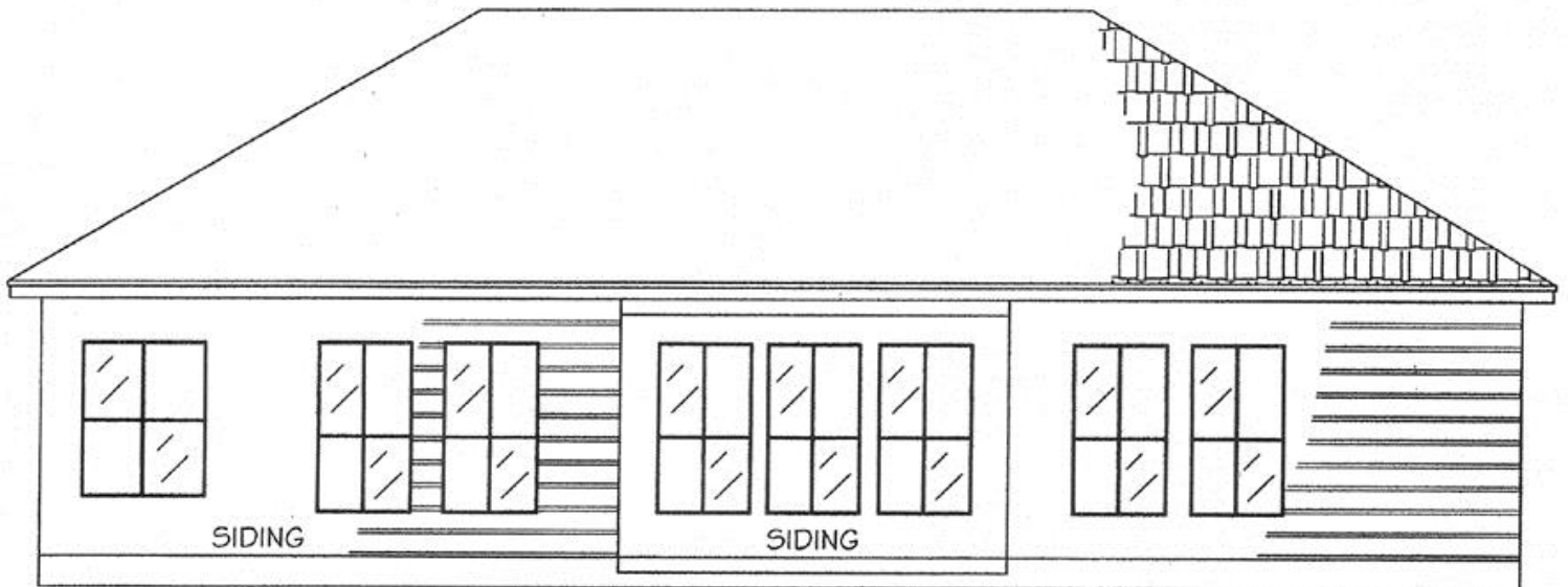
BACK ELEVATION
