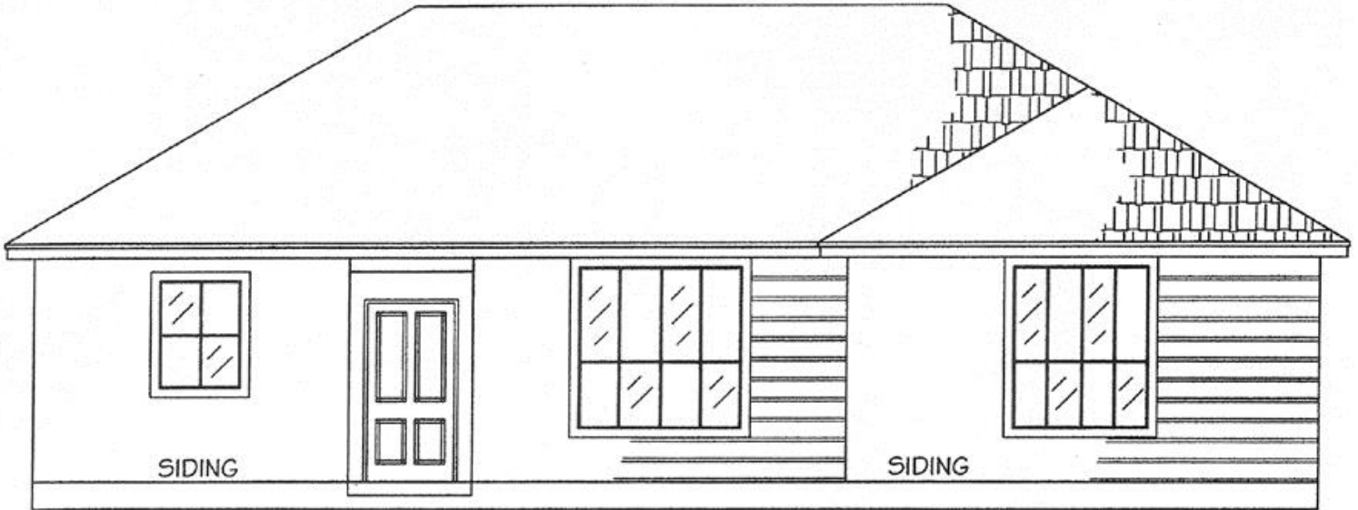
FRONT ELEVATION PLAN No.1227-0705 2-BEDROOM 1-STORY 1227 SQ. FT. LIVING AREA MONTE SMITH DESIGNS COPYRIGHT 2007
