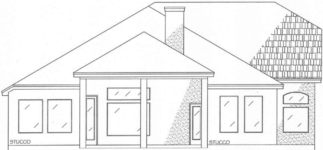
BACK ELEVATION
